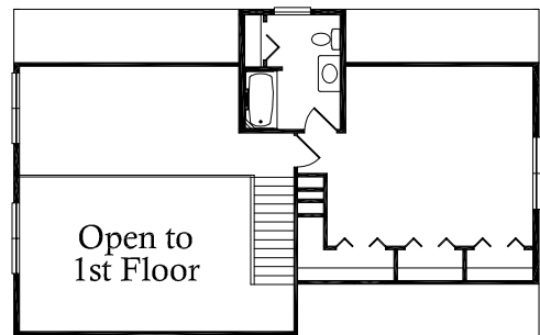
Optional 2nd Floor Layout Finished by others
