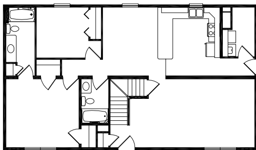
1st Floor Layout with optional "L" staircase
