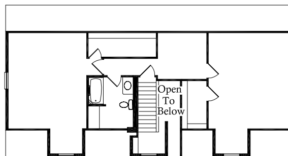
Optional 2nd Floor Layout Finished by others
