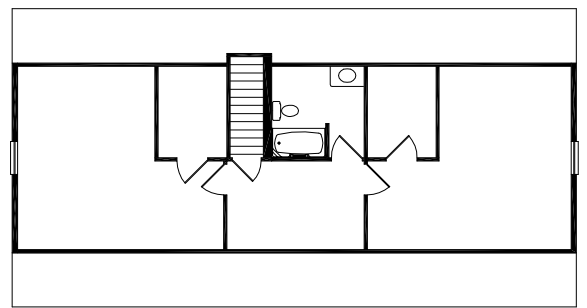
Optional 2nd Floor Layout Finished by others
